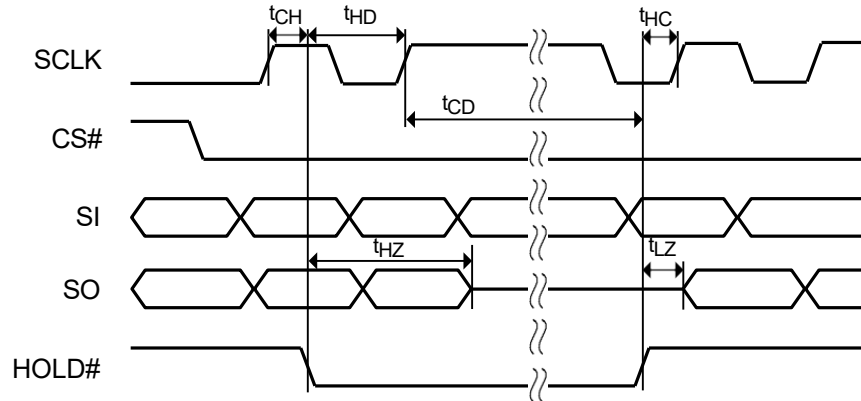
Figure 16-3. Hold# Timing
