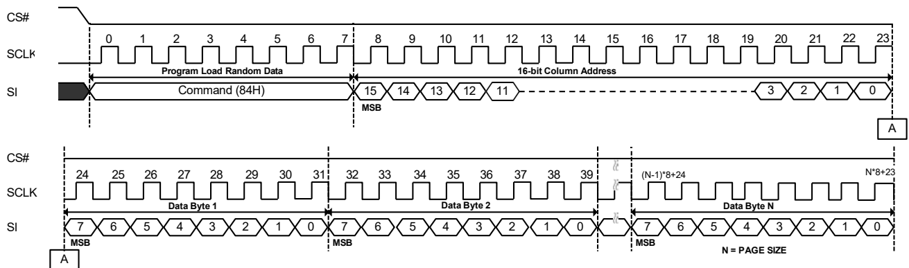
Figure 8-1. Program Load Random Data (84H) Sequence Diagram
